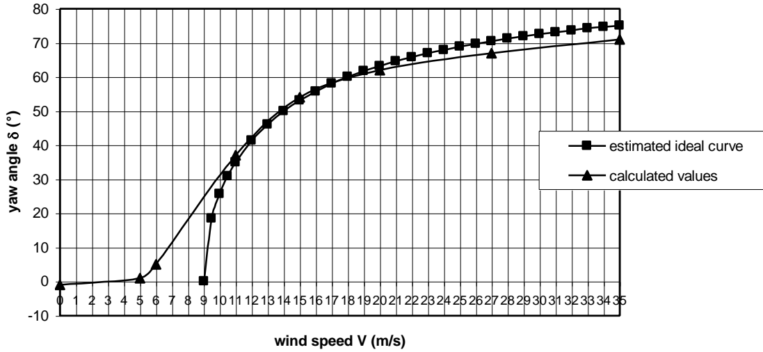
figure 13 The estimated ideal en the calculated \delta -V curve of the VIRYA-3.3D windmill
