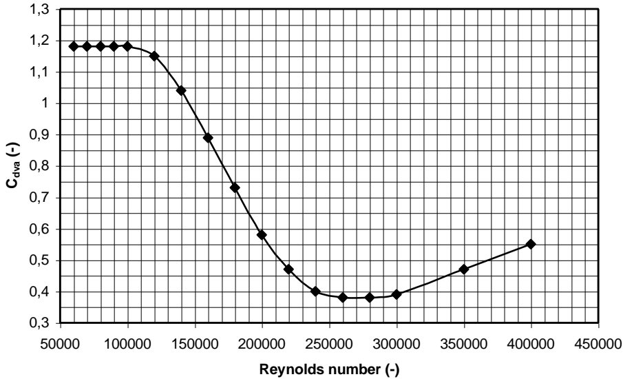
figure 10 Path of C_{dva} as a function of the Reynolds number for a smooth pipe
