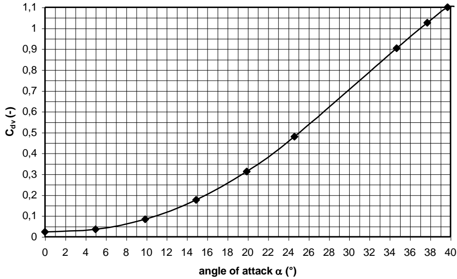
figure 8 Path of C_{dv} as a function of \alpha for a square plate for \alpha < 40^\circ
