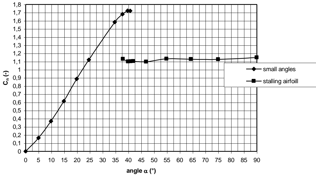
figure 6 Calculated C_n - \alpha curve for a square sheet
