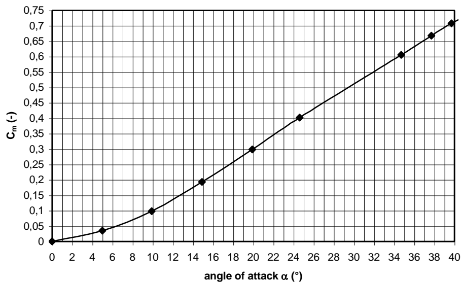
figure 11 Path of C_m as a function of \alpha for a square plate for \alpha < 40^\circ
