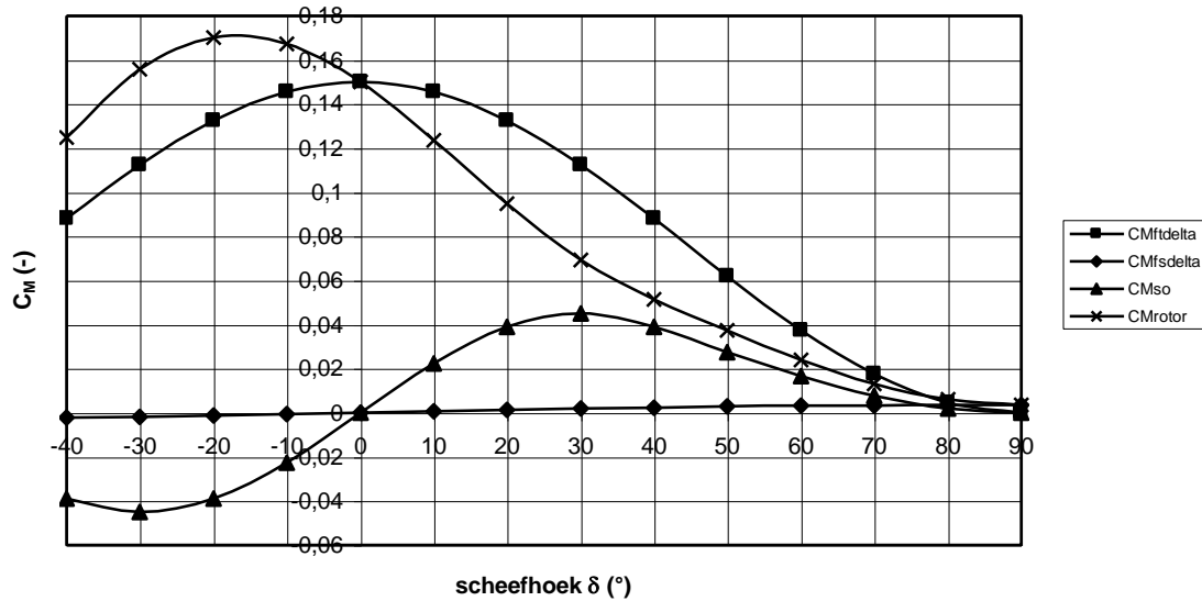
figure 4 Path of C_{MFt\delta} , C_{MFs\delta} , C_{Ms0} and C_{Mrotor} for the VIRYA-3.3D rotor
