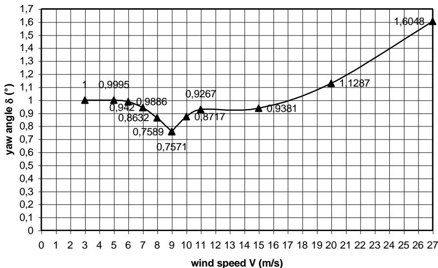
figure 15 Calculated values for \cos^3\delta_{cal} / \cos^3\delta_{id}
