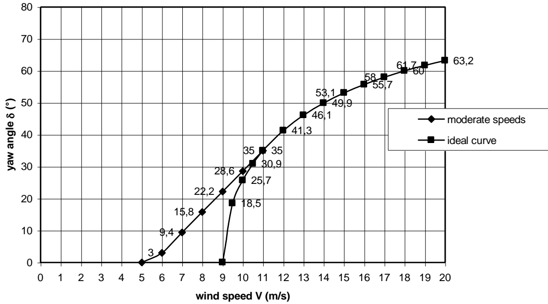
figure 5 Estimated \delta -V curve of the VIRYA-3.3D windmill
