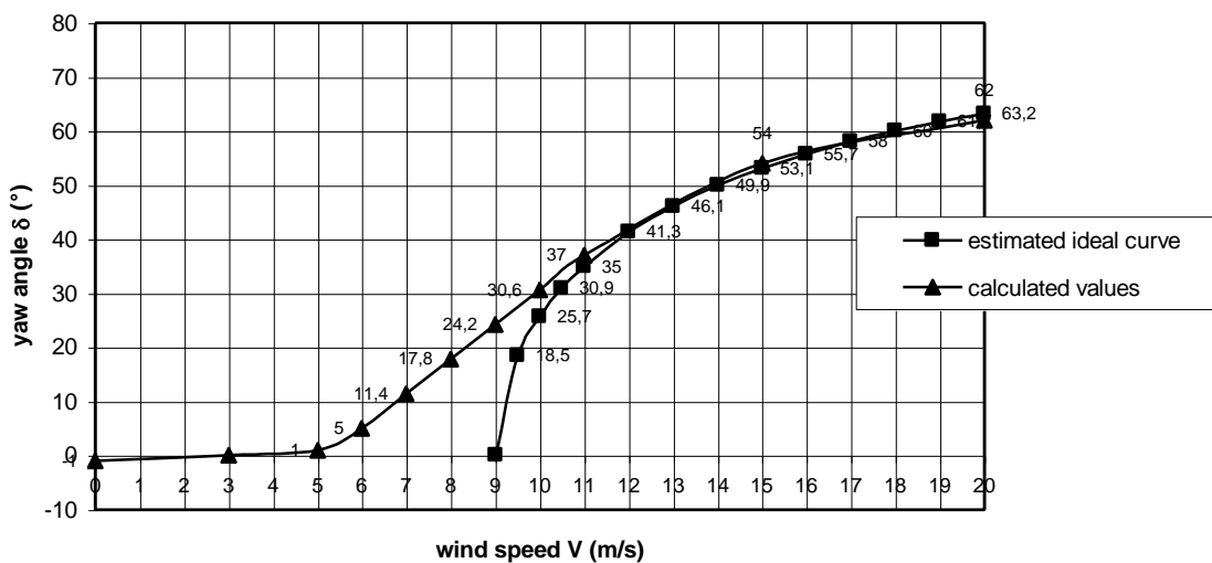
figure 14 The estimated ideal en the calculated \delta -V curve of the VIRYA-3.3D windmill for V < 20 m/s and with added values for the calculated curve for V = 3, 7, 8, 9 and 10 m/s
