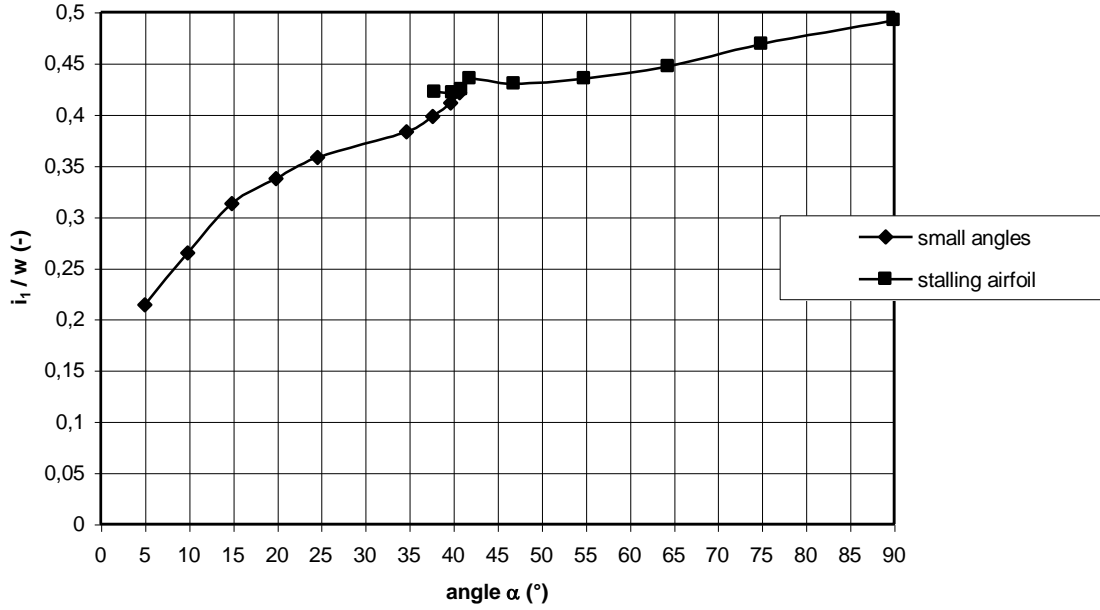
figure 7 Path of i_1 / w as a function of \alpha using N for a square plate.
