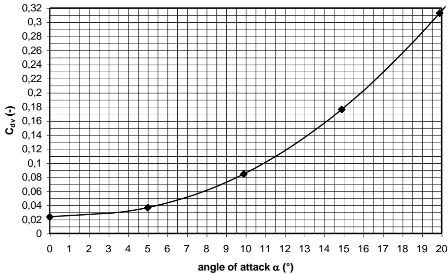
figure 9 Path of C_{dv} as a function of \alpha for a square plate for \alpha < 20^\circ
