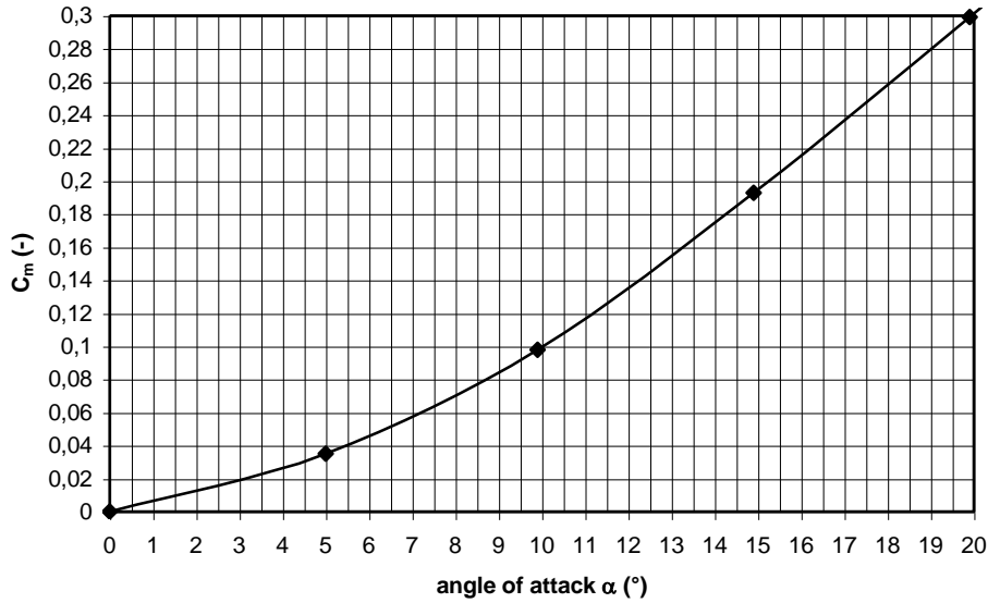
figure 12 Path of C_m as a function of \alpha for a square plate for \alpha < 20^\circ
