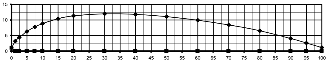
fig. 1 Gö 711-12% airfoil for c = 100 mm
