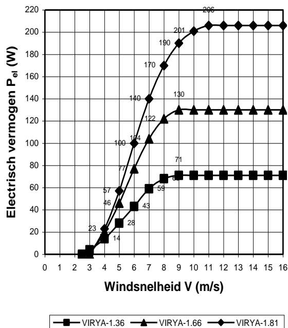
P_{el} -V krommen VIRYA-1.36, VIRYA-1.66 en VIRYA-1.81 windmolens
