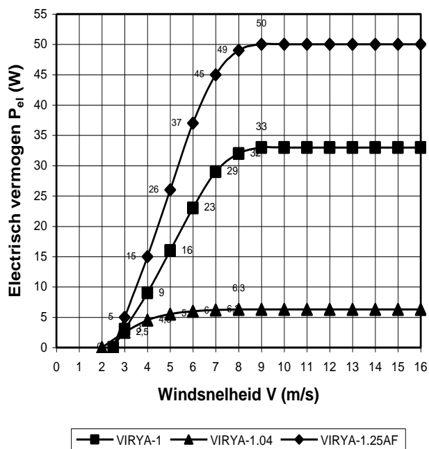
P_{el} -V krommen VIRYA-1, VIRYA-1.04 en VIRYA-1.25AF windmolens
