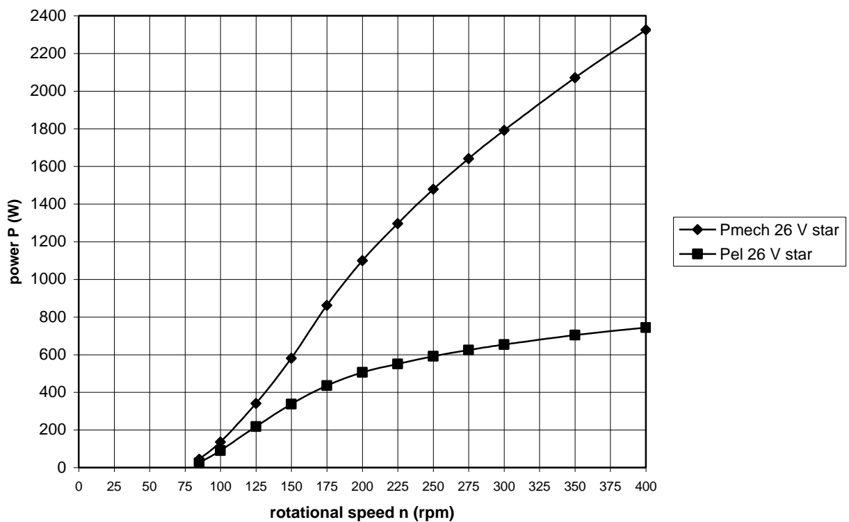
fig. 22 Estimated P_{\text{mech}}-n and P_{\text{el}}-n curves for 26 V star
