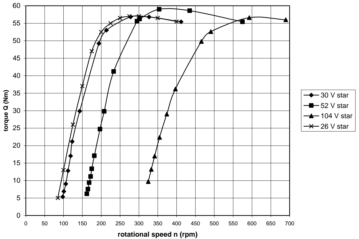
fig. 6 Measured torque Q as a function of n for U = 30 V, U = 52 V and U = 104 V in star. Estimated torque Q as a function of n for U = 26 V star
