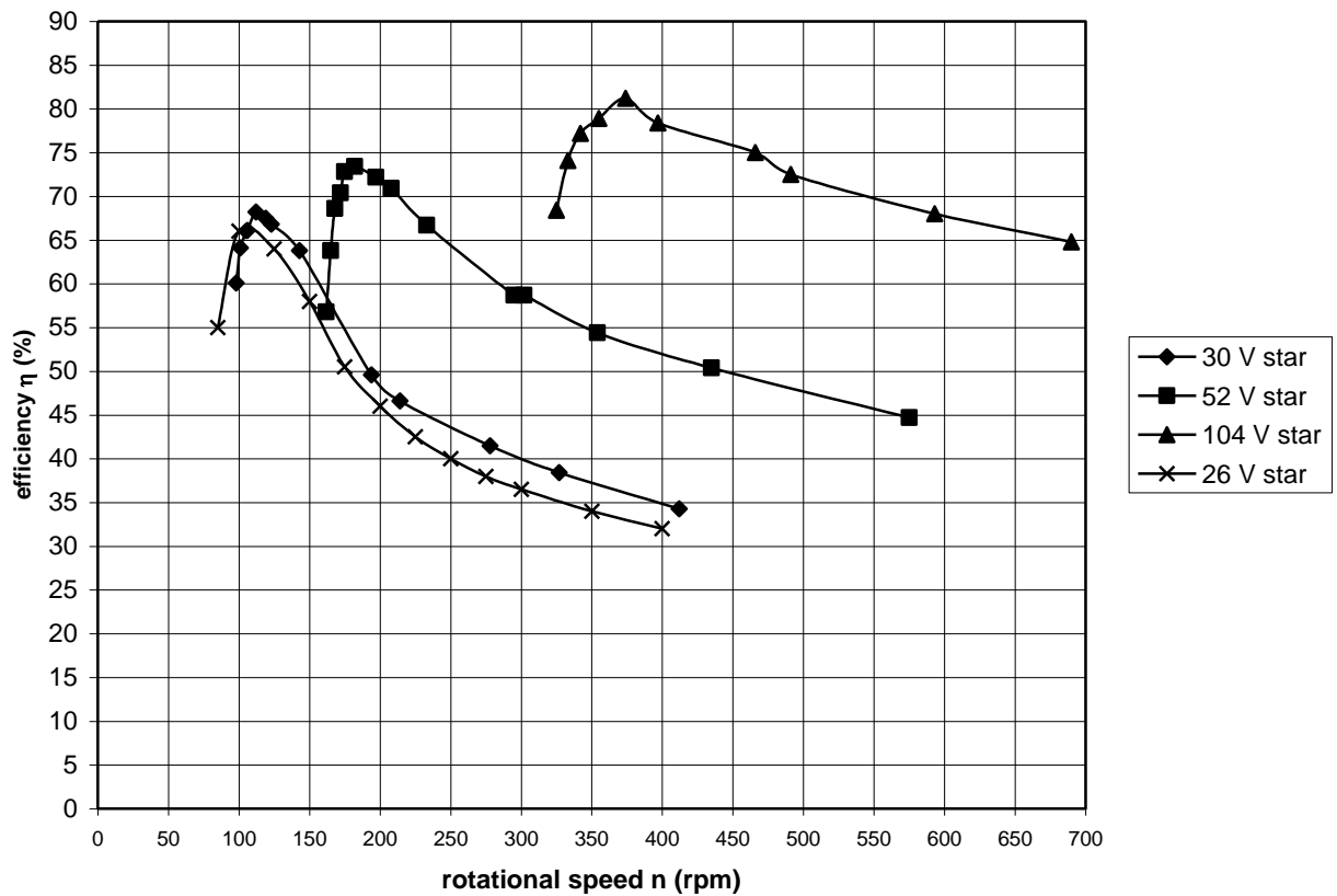
fig. 8 Efficiency \eta as a function of n for U = 30 V, U = 52 V and U = 104 V in star Estimated efficiency \eta as a function of n for U = 26 V star
