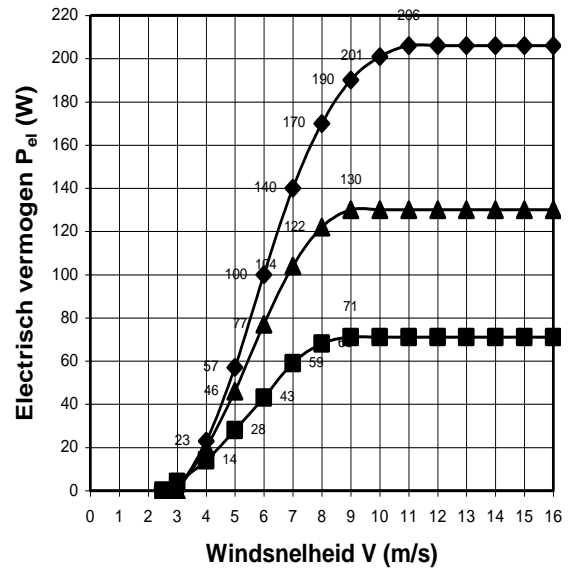
P_{el} -V krommen VIRYA-1.36, VIRYA-1.66 en VIRYA-1.81 windmolens
