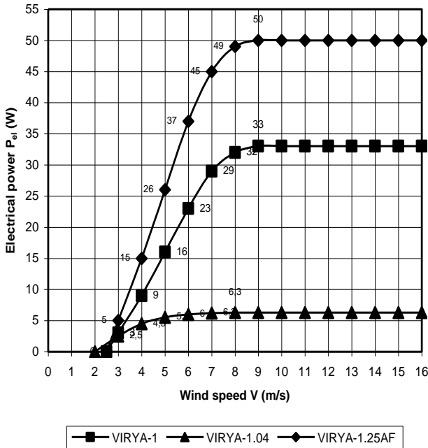
P_{el} -V curves VIRYA-1, VIRYA-1.04 and VIRYA-1.25AF windmills
