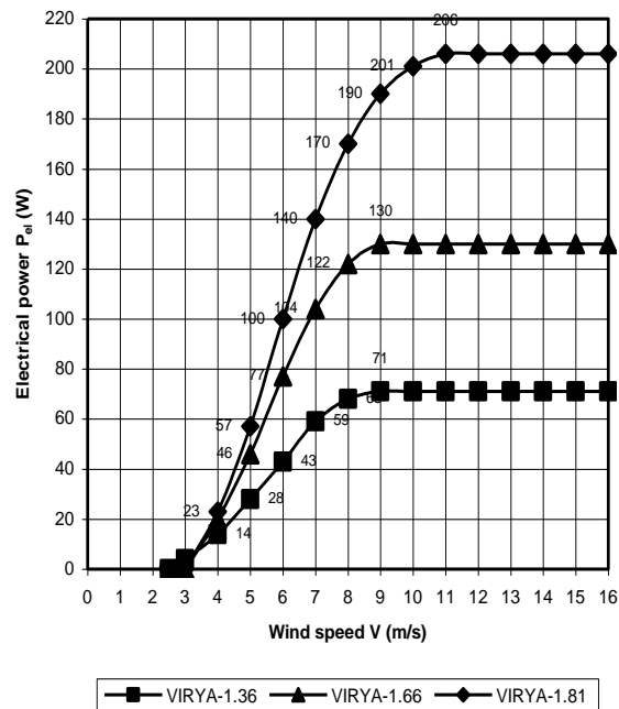
P_{el} -V curves VIRYA-1.36, VIRYA-1.66 and VIRYA-1.81 windmills
