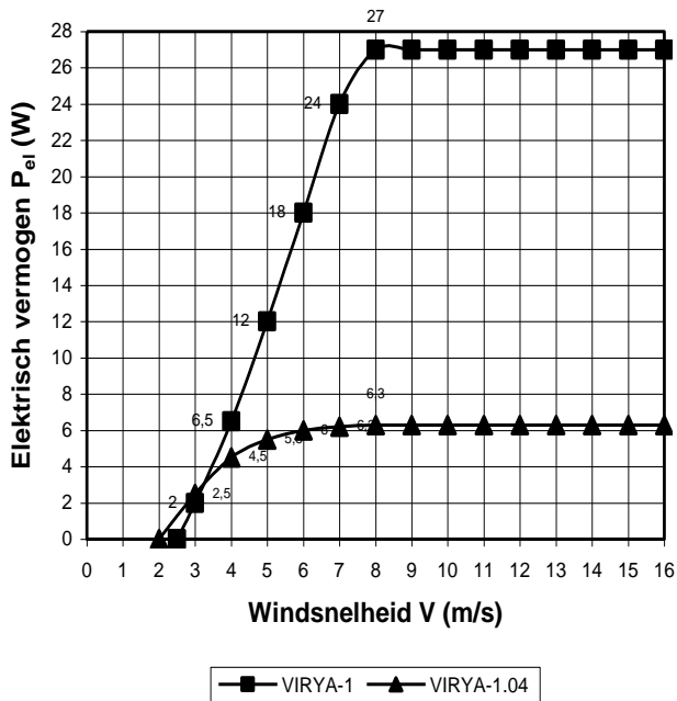
P_{el} -V krommen VIRYA-1 en VIRYA-1.04 windmolens
