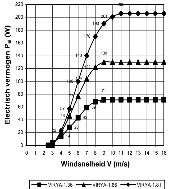
P_{el} -V krommen VIRYA-1.36, VIRYA-1.66 en VIRYA-1.81 windmolens
