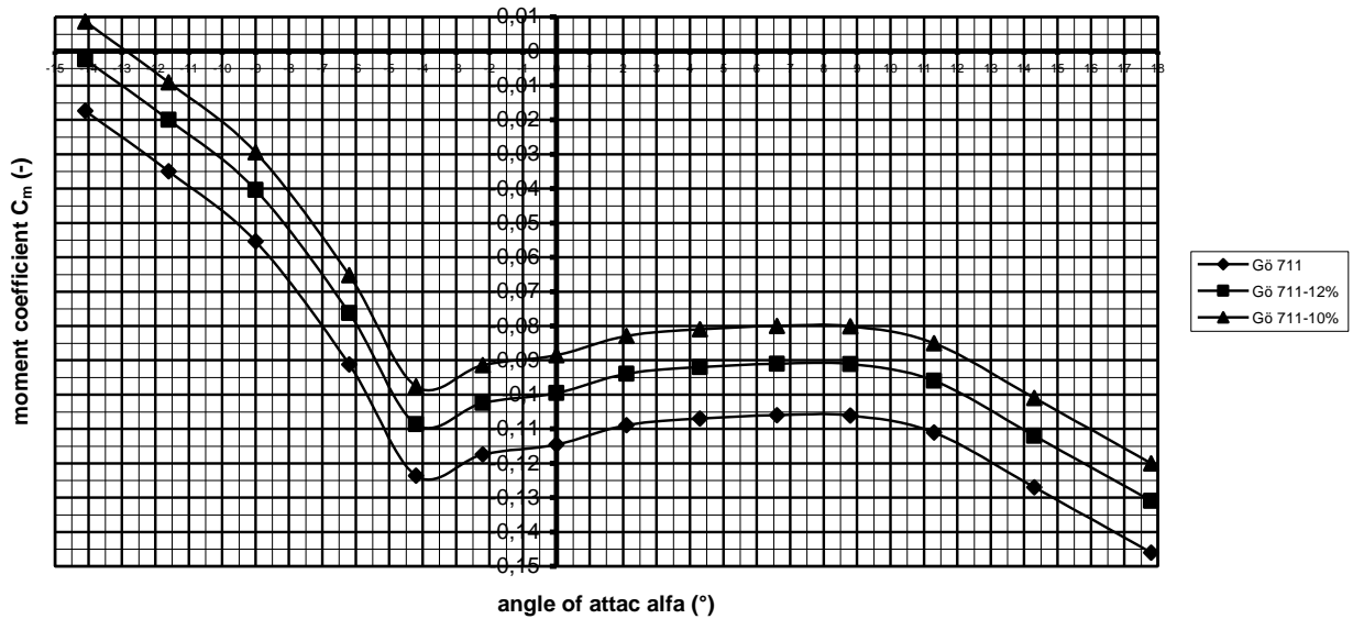
fig. 8 Measured C_m - \alpha curve for the Gö 711 airfoil and estimated C_m - \alpha curve for the Gö 711-12% and Gö 711-10% airfoils for Re = 4 * 10^5
