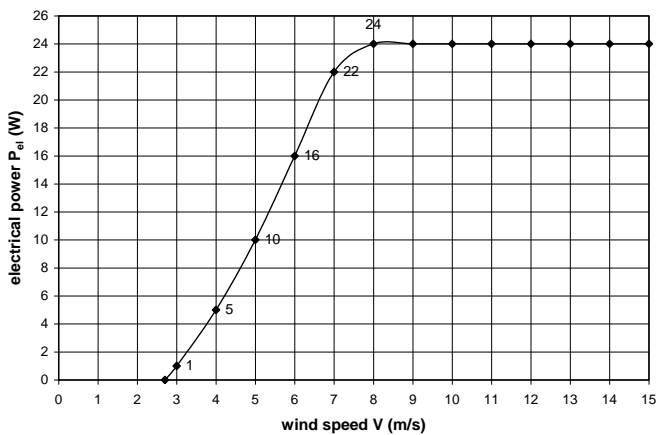
P el -V curve VIRYA-1.02 windmill
