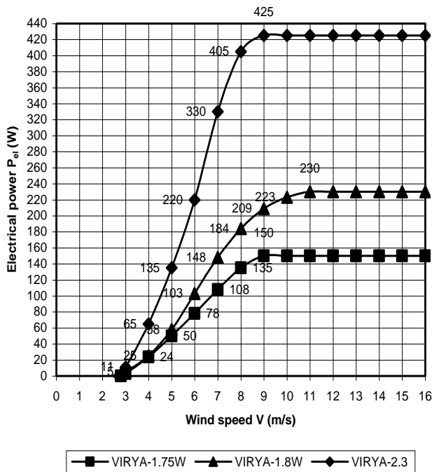
P el -V curves VIRYA-1.75W, VIRYA-1.8W and VIRYA-2.7 windmills
