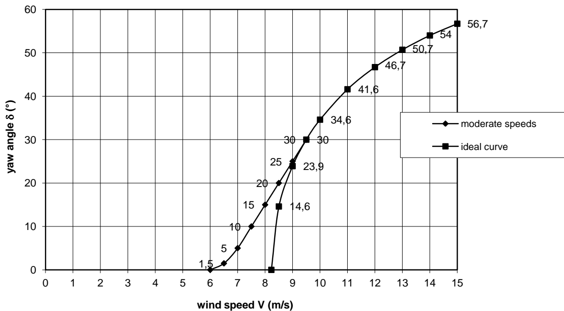
fig. 3 \delta -V curve VIRYA-3B3 safety system with V_{rated} = 9.5 \text{ m/s}
