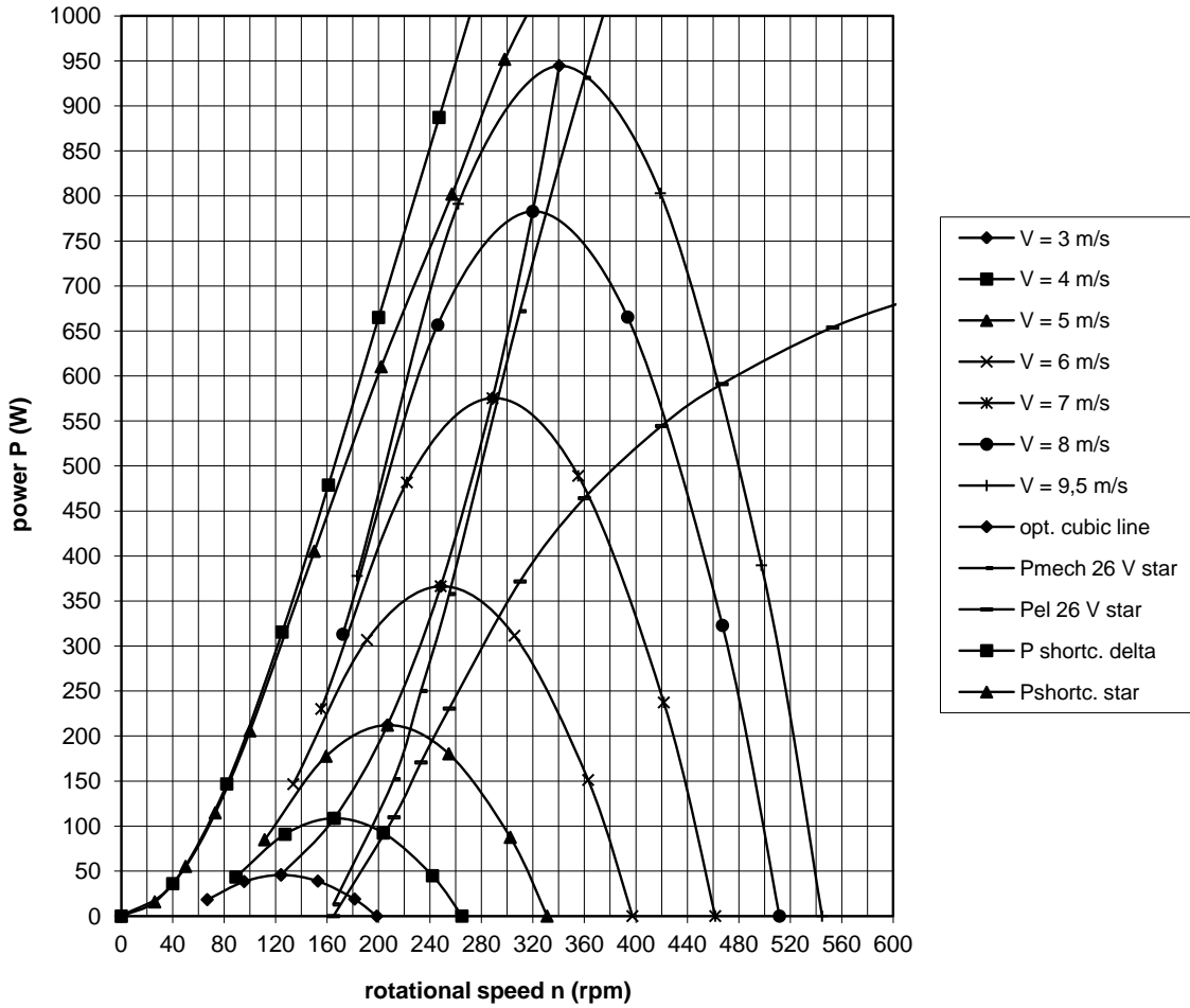
fig. 4 P-n curves of the VIRYA-3B3 rotor for V_{rated} = 9.5 m/s, optimum cubic line, P_{mech} -n and P_{el} -n curves of the generator with modified 115/200 V winding for 26 V star and P-n curves of the generator for short-circuit in delta and star.
