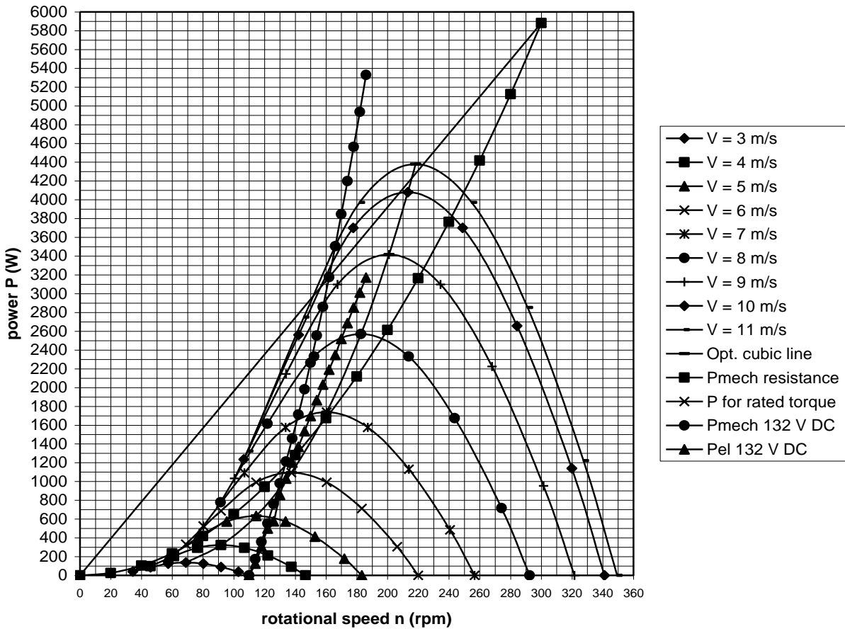
fig. 10 P-n curves of the VIRYA-5B3 rotor, optimum cubic line, P_{\text{mech}} -n curve for the generator with a resistance load such that P_{\text{el}} = 5000 \text{ W} at n = 300 \text{ rpm} , P-n curve for the rated torque, P_{\text{mech}} -n and P_{\text{el}} -n curves for 132 V DC
