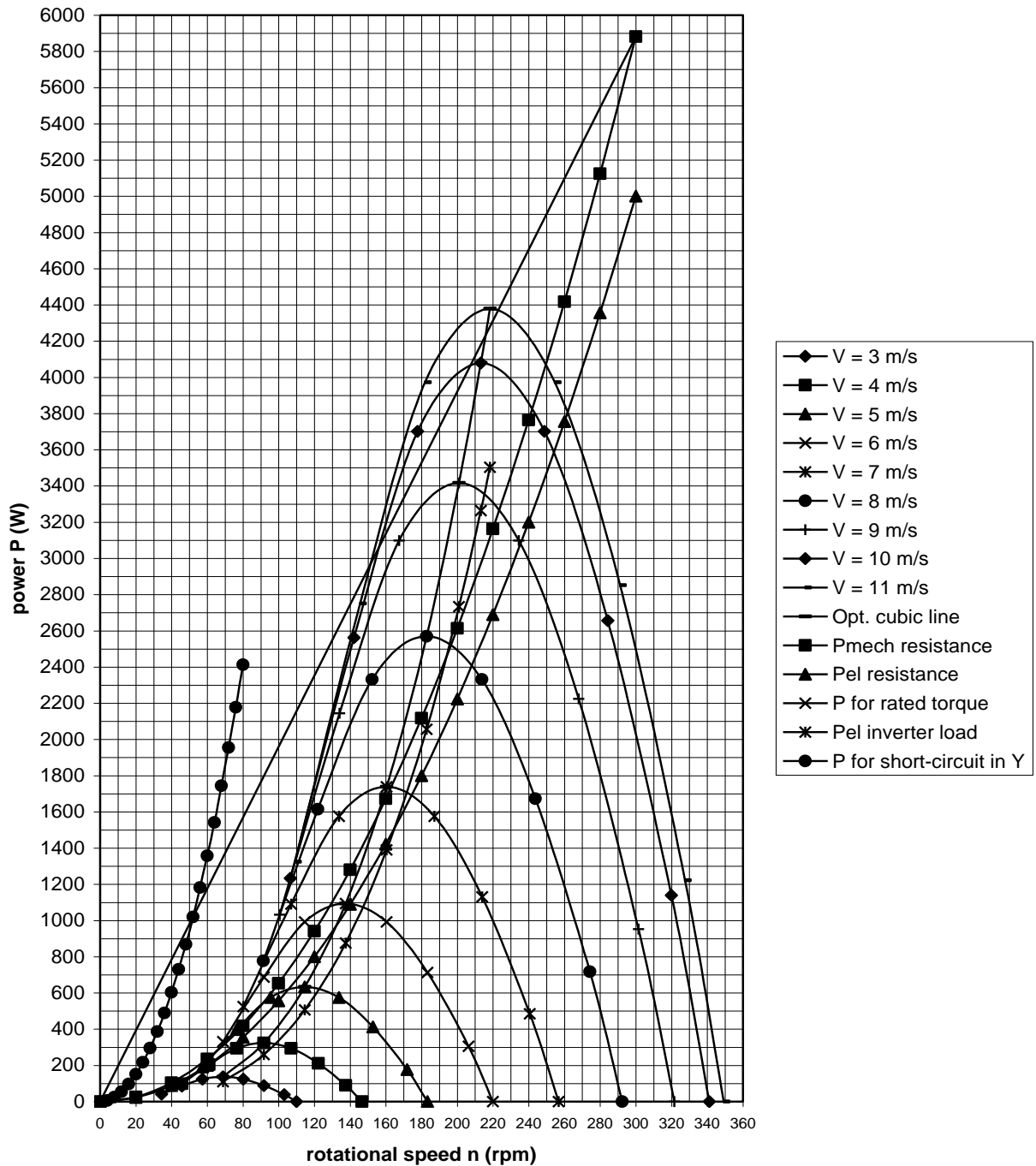
fig. 5 P - n curves of the VIRYA-5B3 rotor, optimum cubic line, P_{\text{mech}} - n and P_{\text{el}} - n curves for the generator with a resistance load such that P_{\text{el}} = 5000 W at n = 300 rpm, P - n curve for the rated torque, P_{\text{el}} - n curve for an inverter load, P - n curve for short-circuit in star
